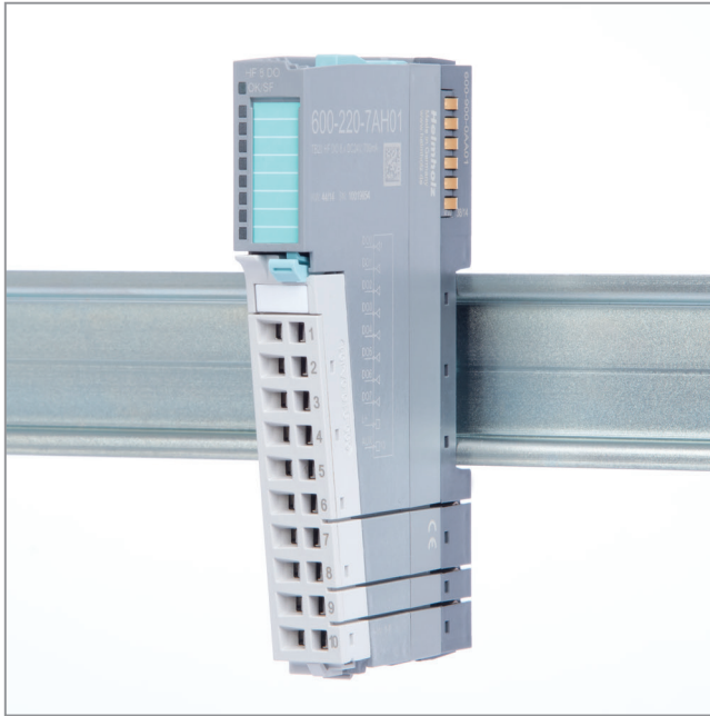
DO 8 x 24 VDC, 700 mA, Highfeature
