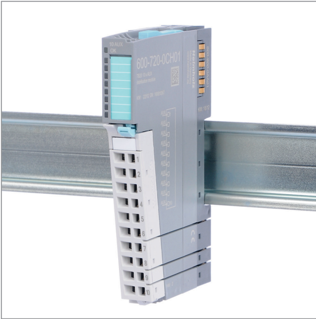
Potential distributor 10 x AUX
