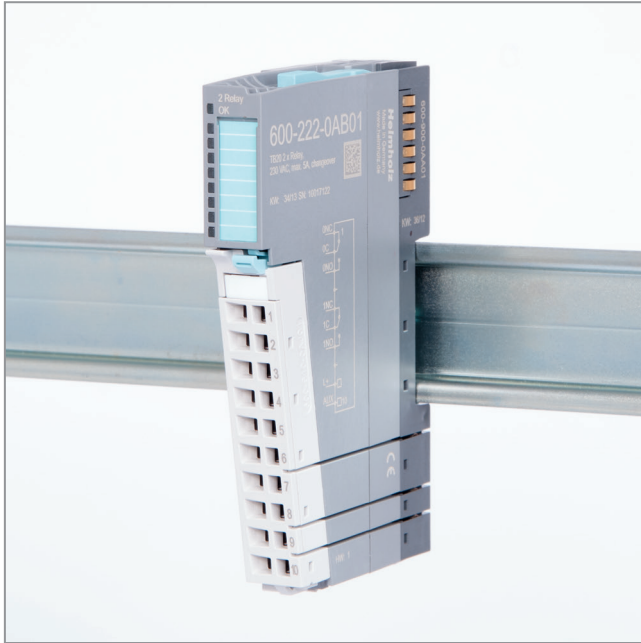
DO 2 x relays, 5 A, 230 VAC, changeover
