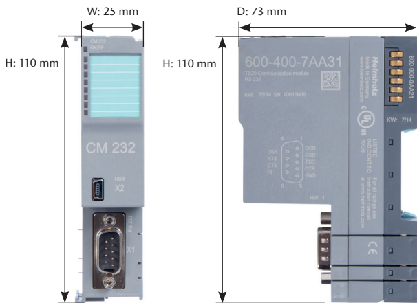
Communication module
