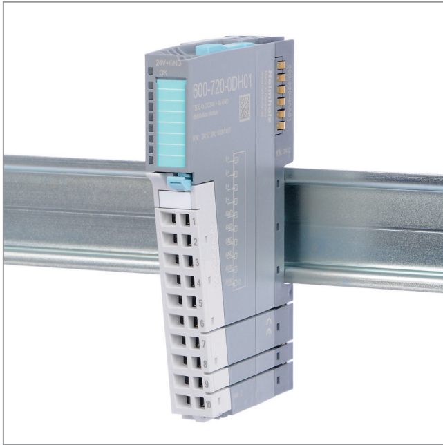
Potential distributor 4 x 24 VDC + 4 x GND
