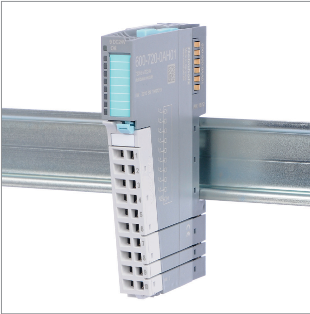
Potential distributor 9 x 24 VDC
