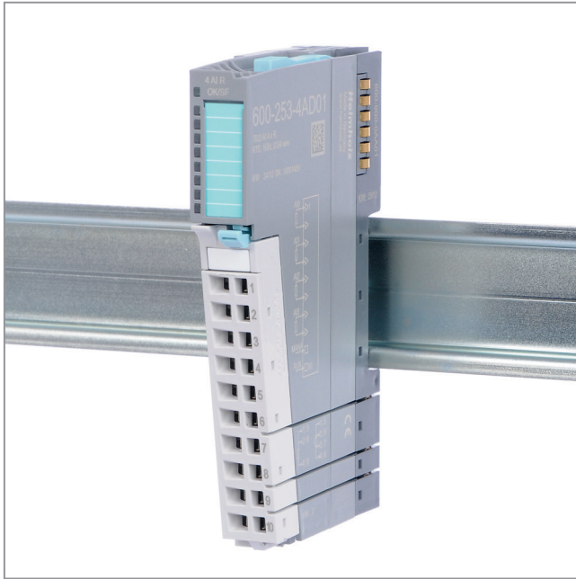
AI 2/4 x R, RTD, 16 Bit, 2/3/4-wire
