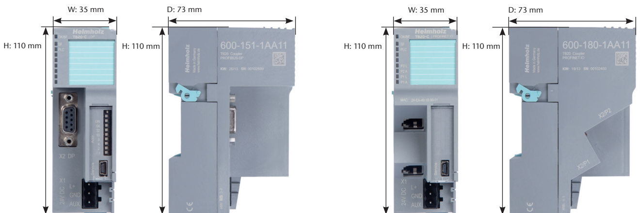
Bus Couplers
