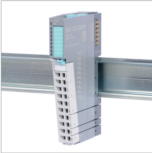
Potential distributor 9 x GND
